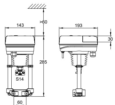
Fig 7: VAP3000L
