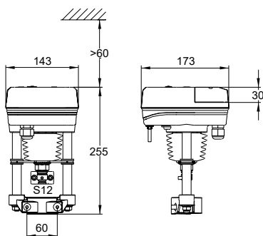
Fig 5: VAP600S / VAP1000S
