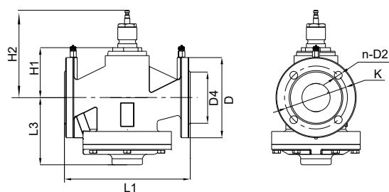
Fig 4: DN65-DN250
