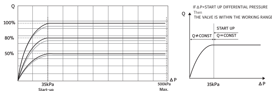
Fig 1: Dynamic Characteristic Curves
