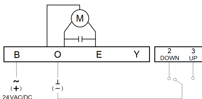
Fig 6: Floating Application
