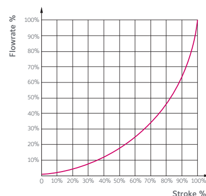
Fig 2: Flow characteristic - equal percentage
