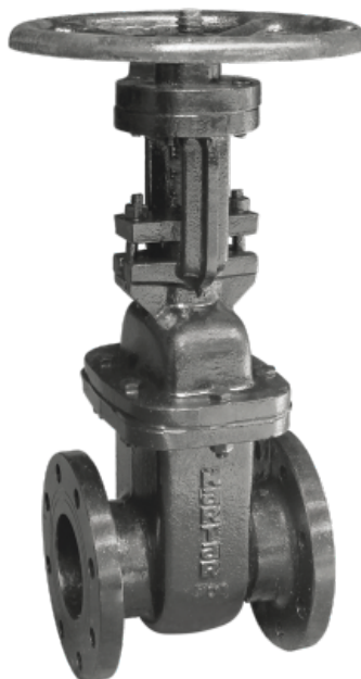
OS&Y TYPE (Rising Stem) K 505, 506
